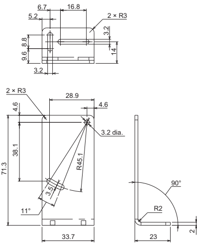
Mounting bracket
