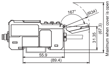
Cover open position (DIN Track mounting)
